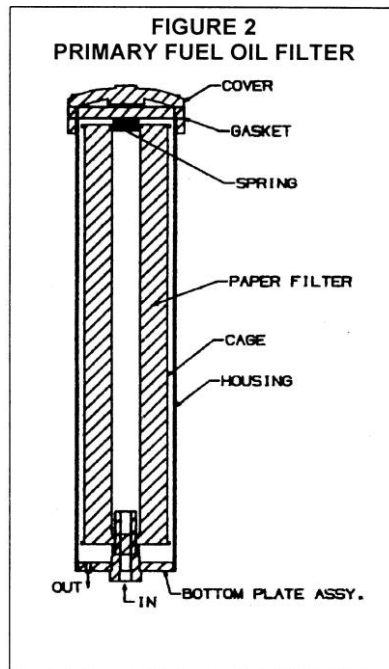
PRIMARY FUEL OIL FILTER
