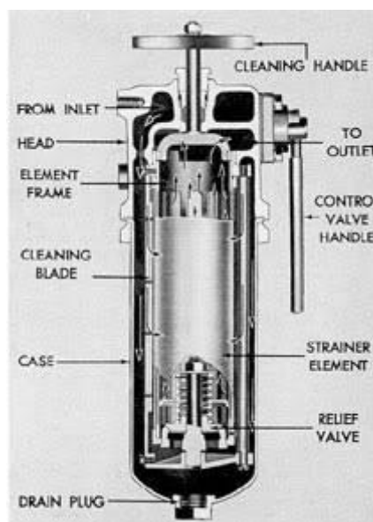
LUBE OIL STRAINER
