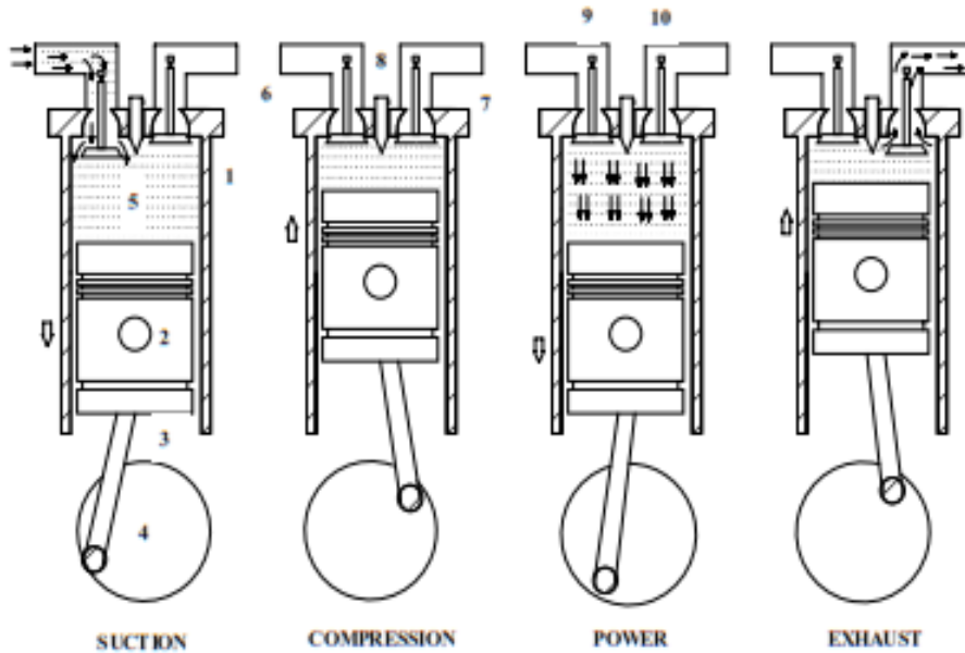
FOURSTROKE CYCLE ENGINE WORKING PRINCIPLE
