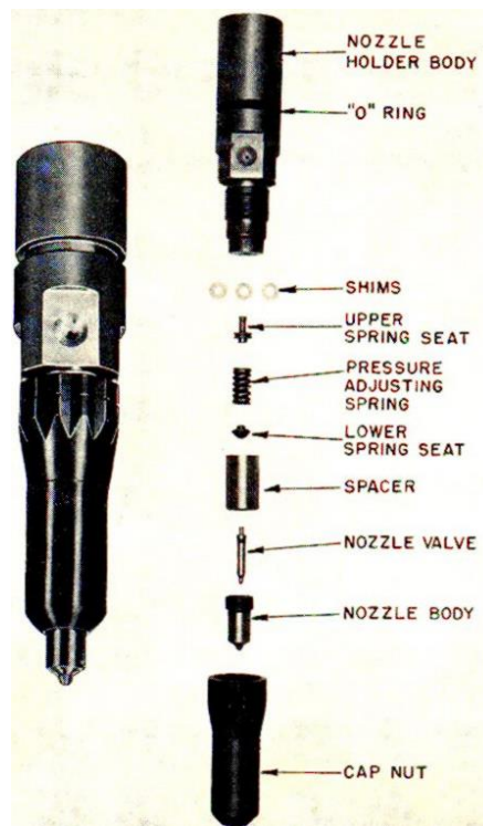
INJECTOR
