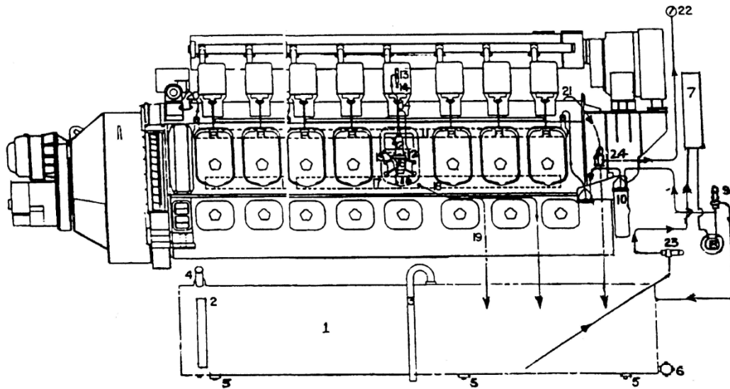
FIGURE 1 NUMBERING SEQUENCE INDICATES OIL FLOW THROUGH THE SYSTEM
