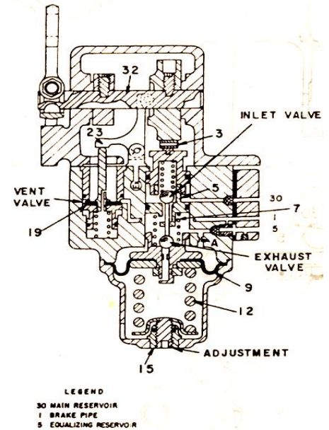
A9-AUTOMATIC BRAKE VALVE
