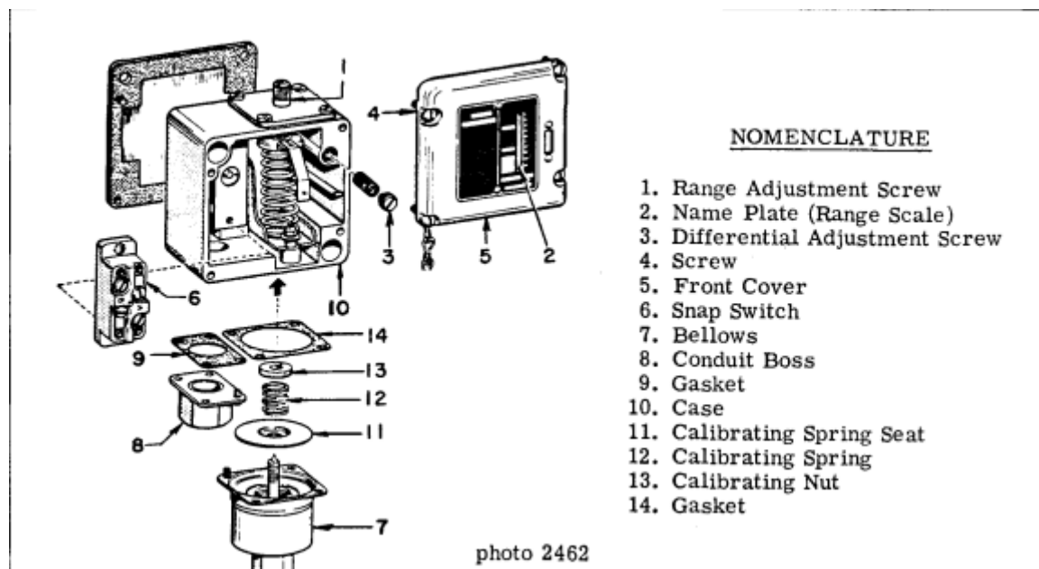
LOW LUBE OIL PRESSURE SWITCH
