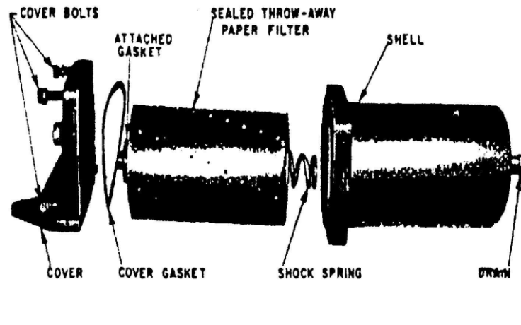
SECONDARY FUEL OIL FILTER
