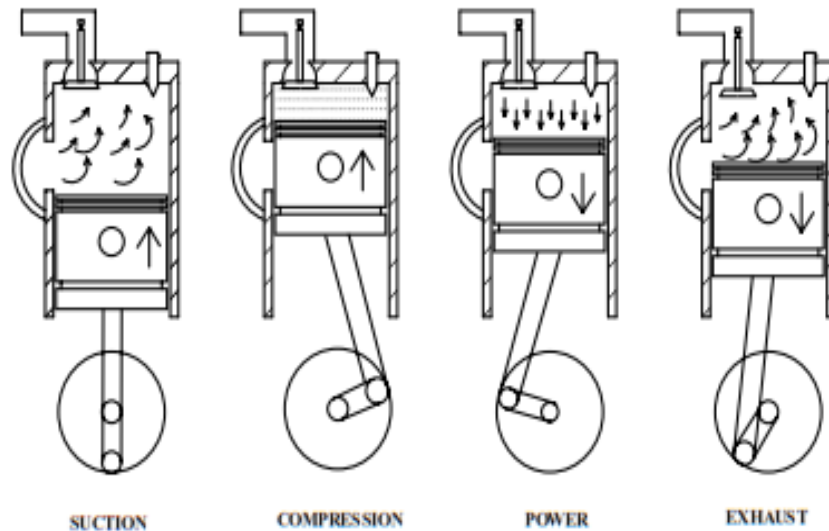
TWO STROKE CYCLE ENGINE WORKING PRINCIPLE
