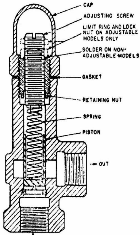
FUEL RELIEF AND REGULATING VALVE
