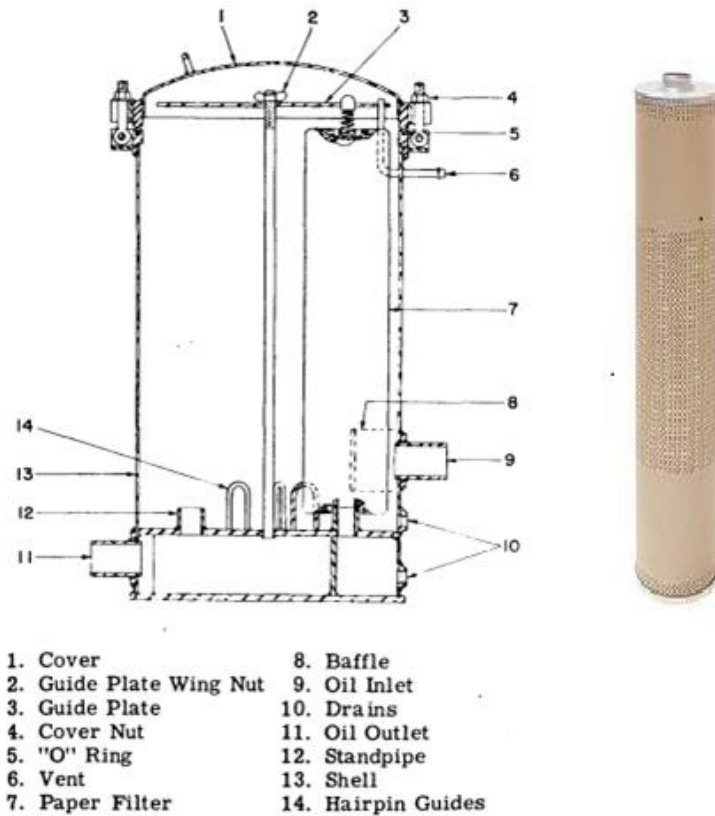
Paper type lube oil filter
