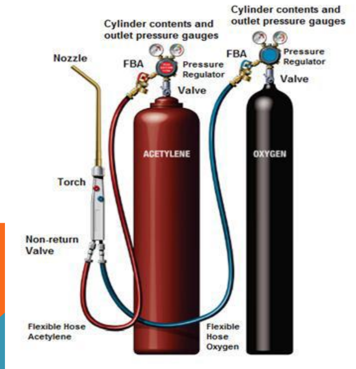
Oxy Acetylene Gas Cutting Equipment
