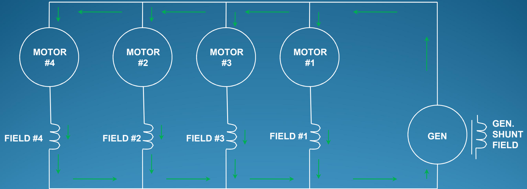
PARALLEL MOTORING CIRCUIT
