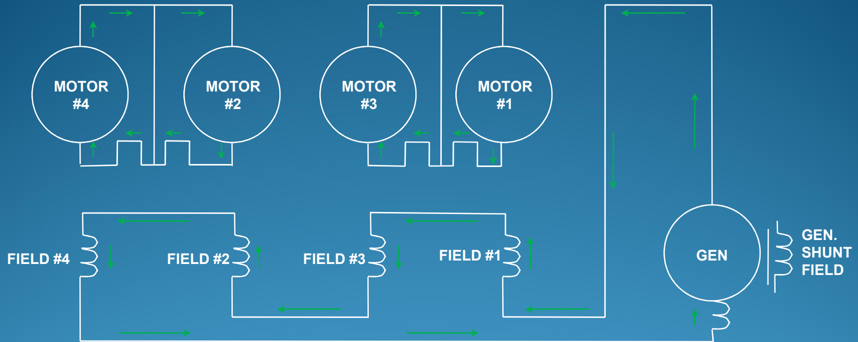
DYNAMIC BRAKING CIRCUIT
