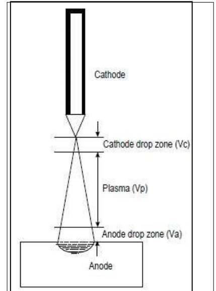
Fig.3 Three different zones in which voltage drop
