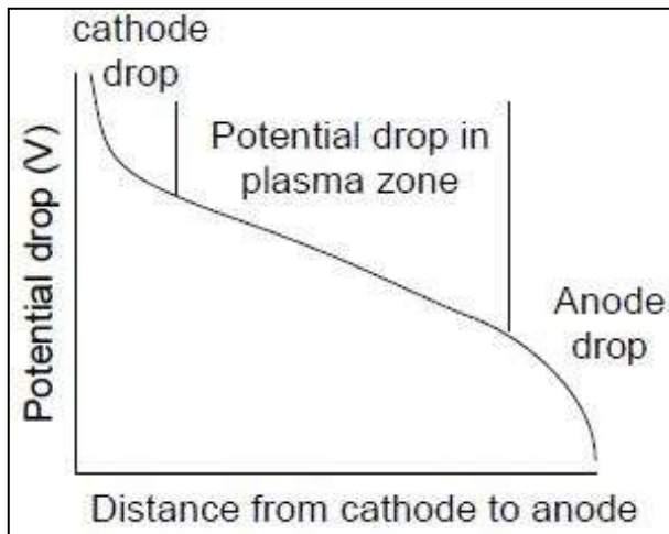
Fig.1 Potential drop as function of distance from the cathode to anode
